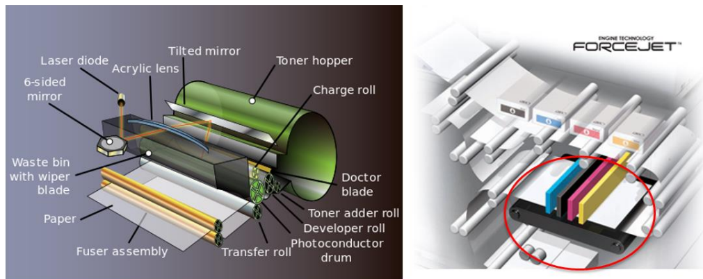
Figure 7: Laser (Left) vs. RISO Inkjet Technology (Right)
