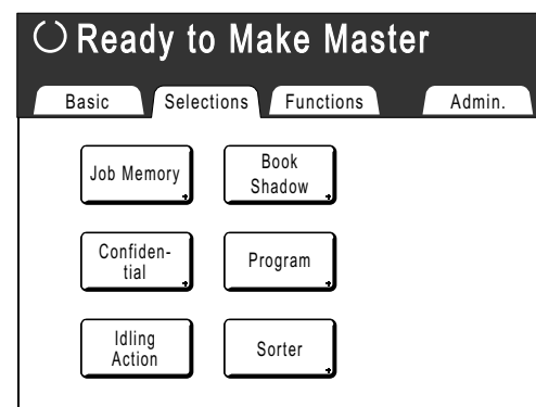
Selections Screen
